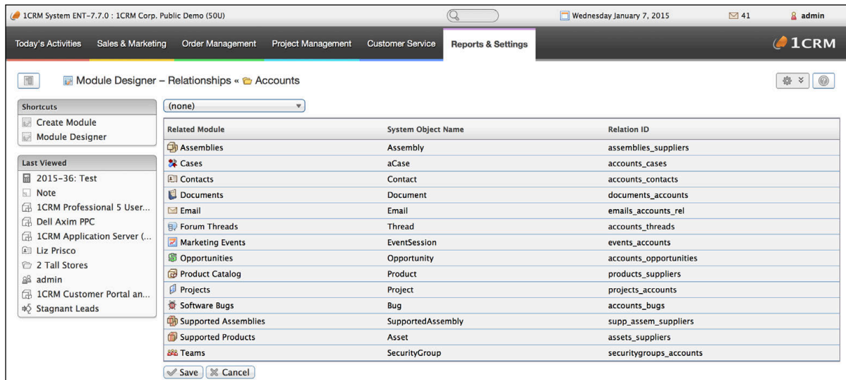
Figure 155: Editing Relationships
