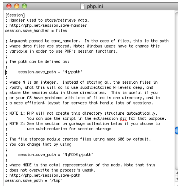
Figure 63: Editing php.ini to Set the Session Save Path
