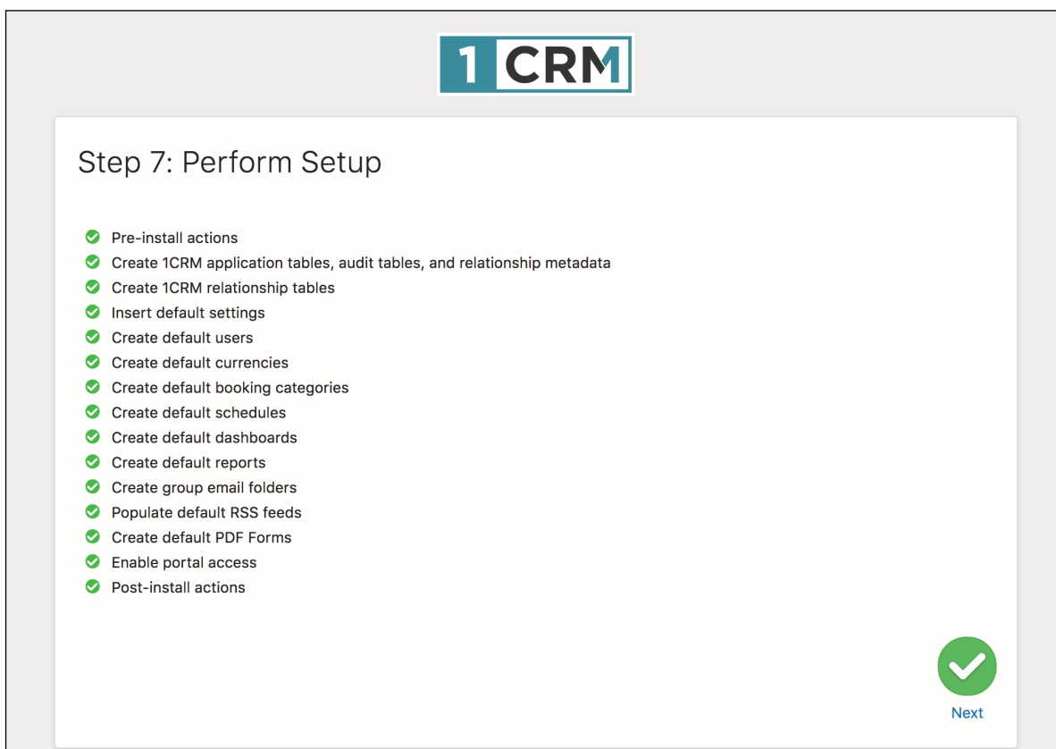
Figure 94: Install Step 7 – Perform Setup (Complete)
